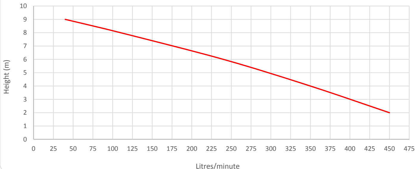
Pump Performance
