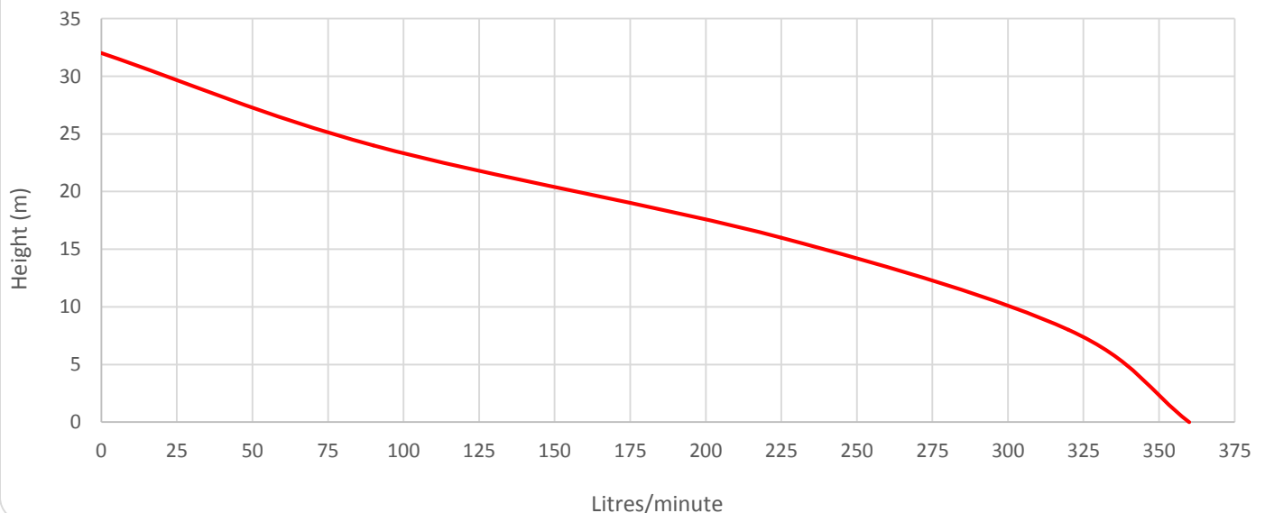
Pump Performance
