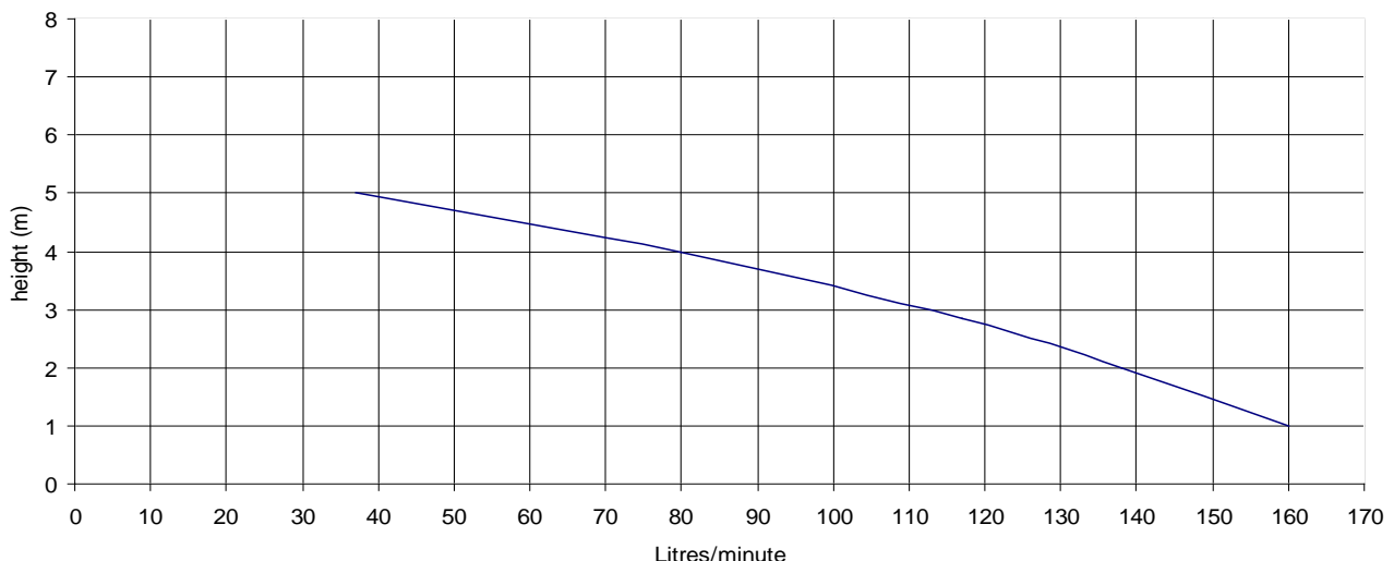
Pump Performance
