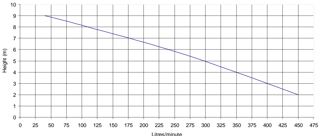
Pump Performance
