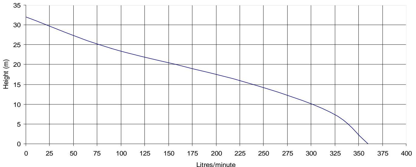
Pump Performance
