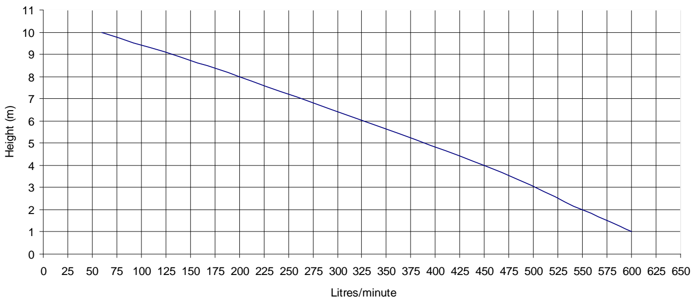
Pump Performance
