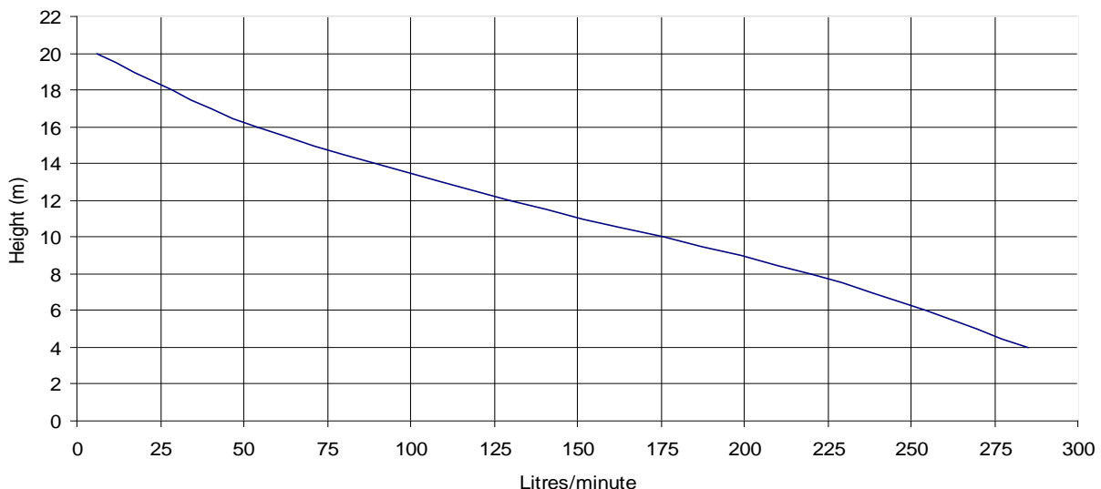
Pump Performance
