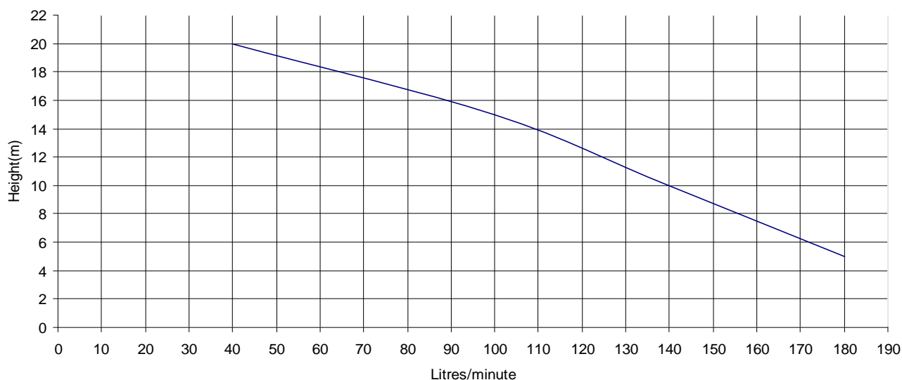
Pump Performance
