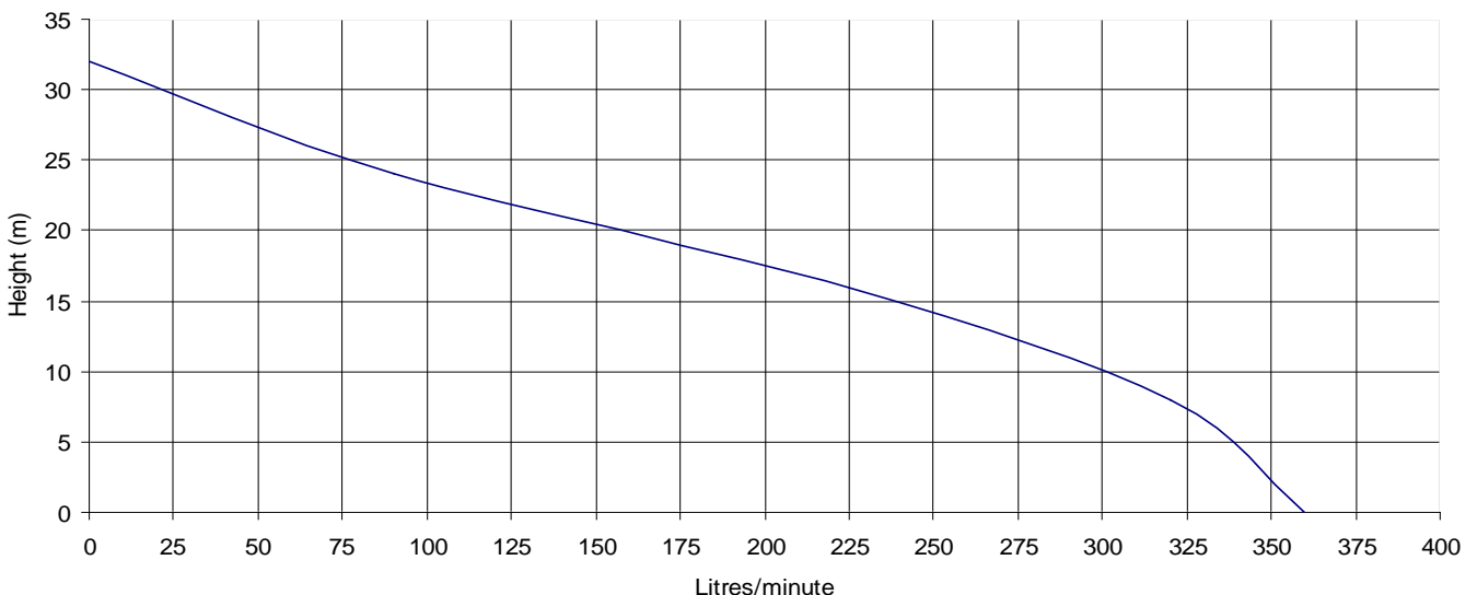
Pump Performance
