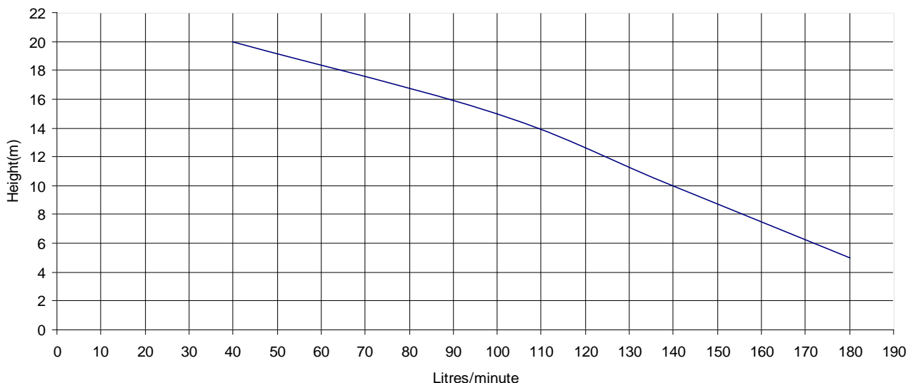
Pump Performance
