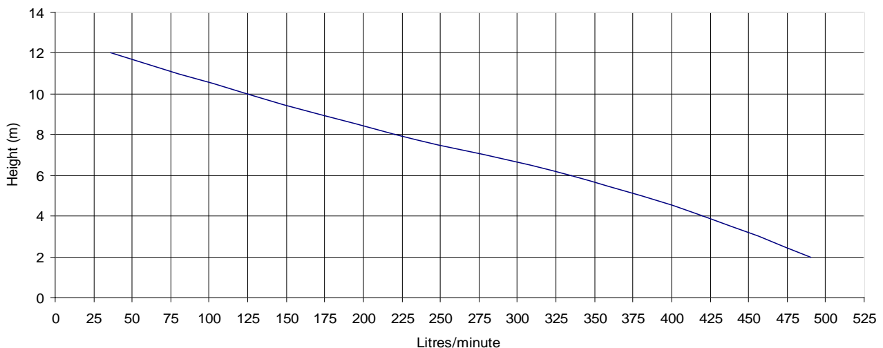
Pump Performance
