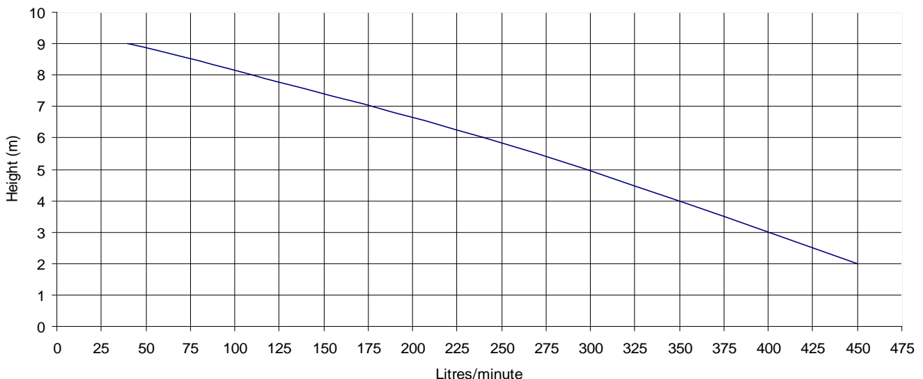
Pump Performance
