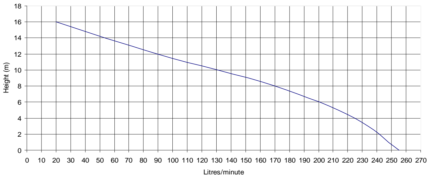
Pump Performance
