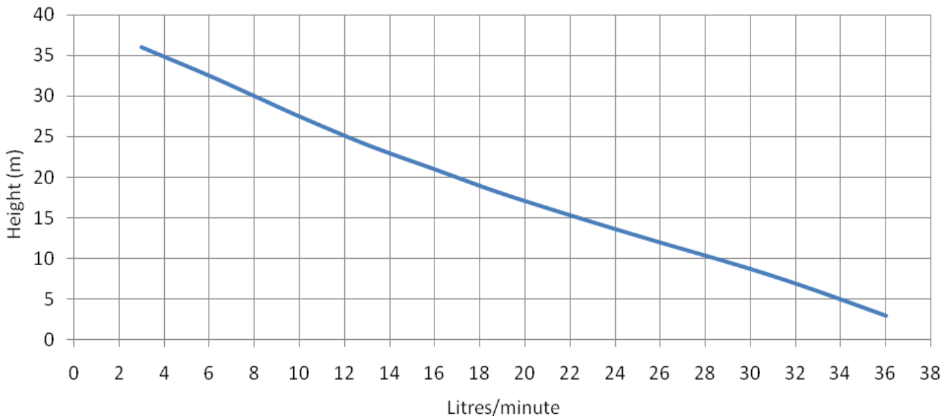
Pump Performance
