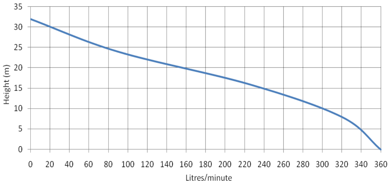
Pump Performance
