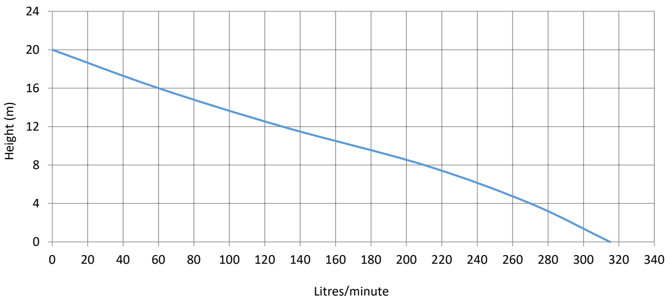
Pump Performance
