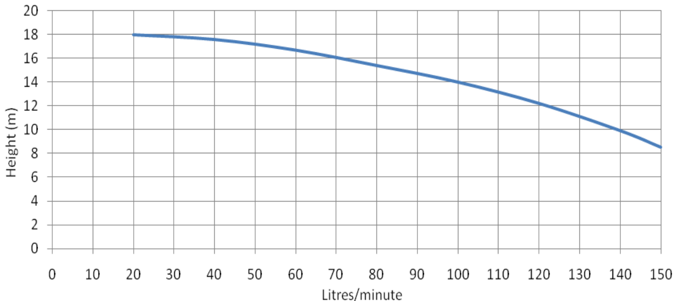
Pump Performance
