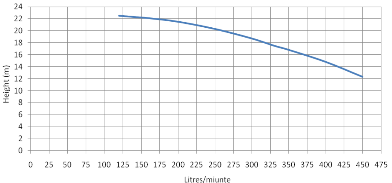
Pump Performance
